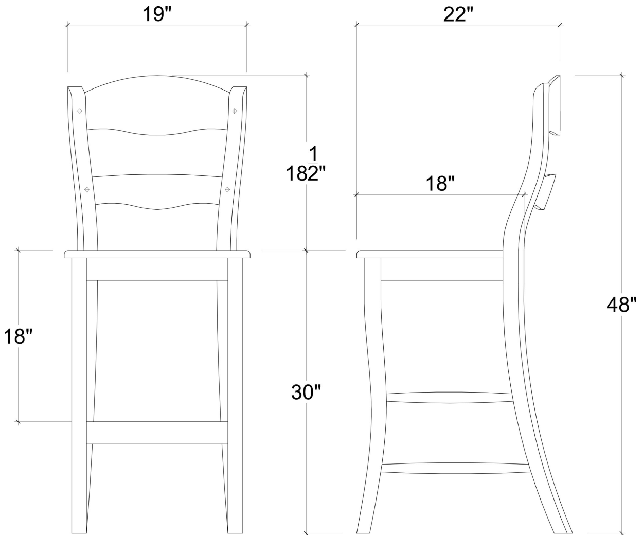
FRONT VIEW
